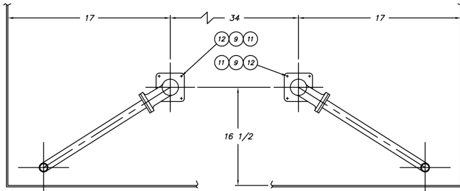
FRONT SECTION A-A
